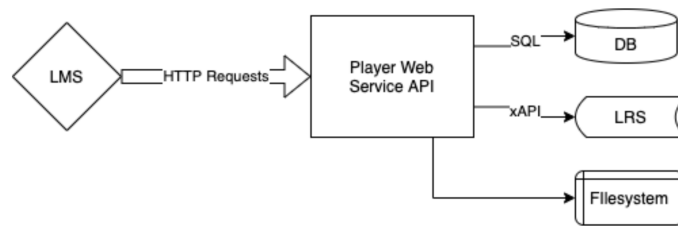
Figure 4. cmi5 Open-Source Content Player Prototype
